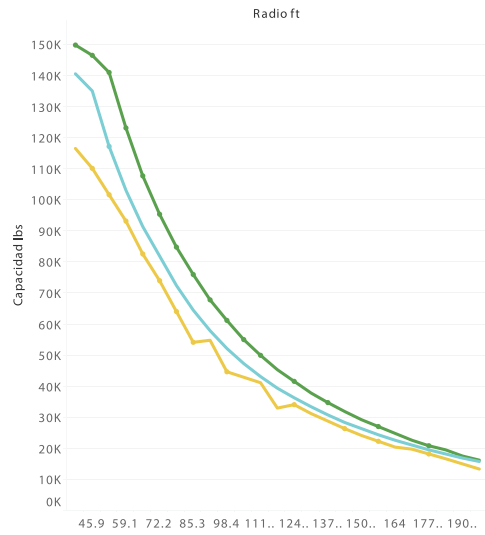
Boom 223.09 ft / lbs
