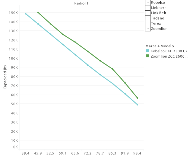
Boom 88.58 ft + Luffi ng 88.58 ft (88°) / lbs
