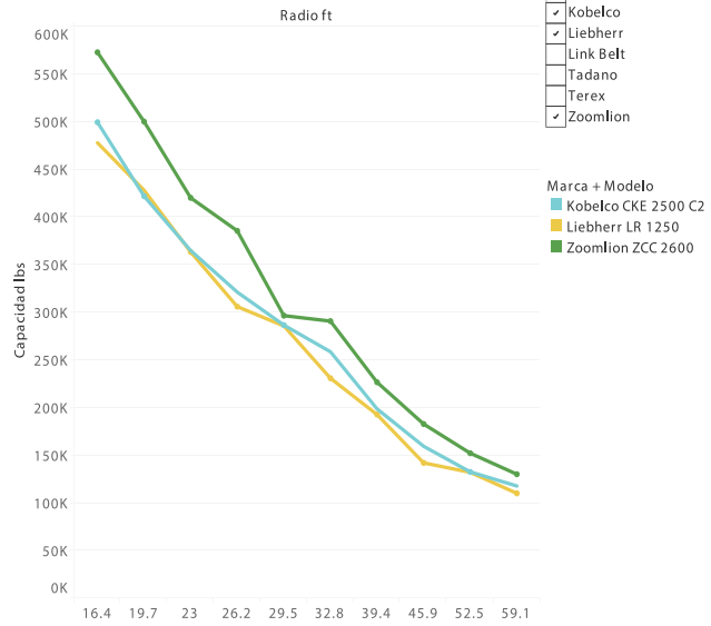
Boom 65.61 ft / lbs
