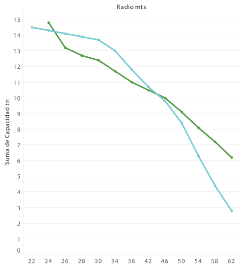
Boom 61m + Luffing 61 m (88°) / tn
