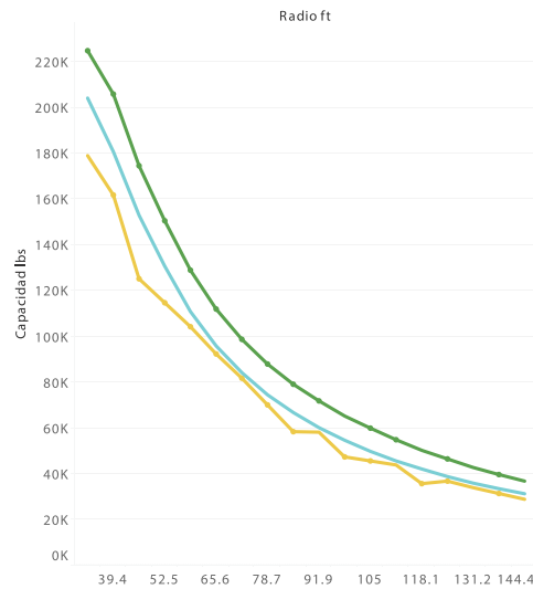
Boom 164.04 ft / lbs
