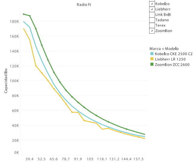
Boom 183.72 ft / lbs
