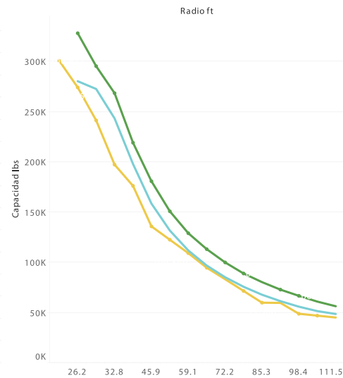
Boom 124.67 ft / lbs
