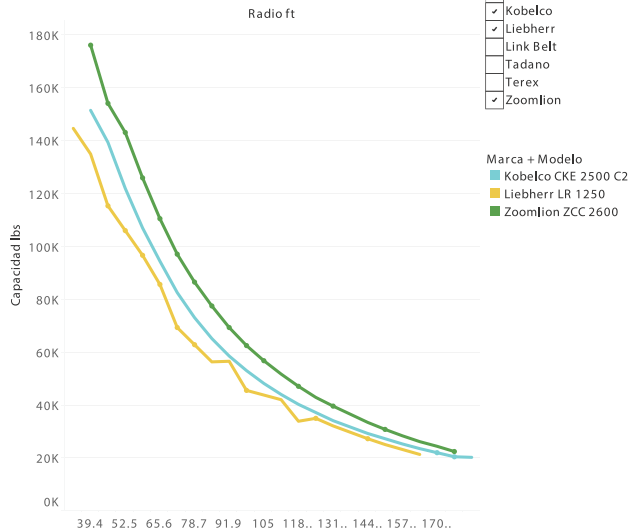
Boom 203.41 ft / lbs
