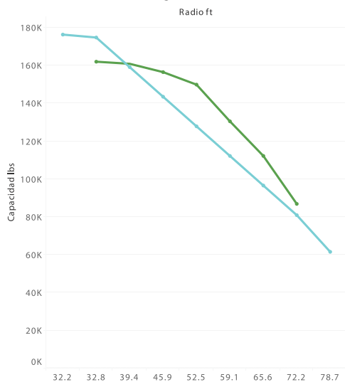
Boom 68.89 ft + Luffi ng 68.89 ft (88°) / lbs
