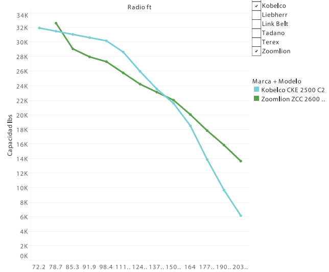
Boom 200.13 ft + Luffing 200.13 ft (88°) / lbs
