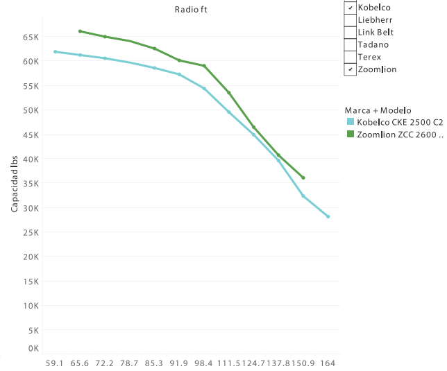
Boom 149.93 ft + Luffing 149.93 ft (88°) / lbs
