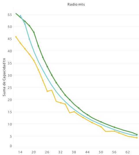
Boom 74 mts / tn
