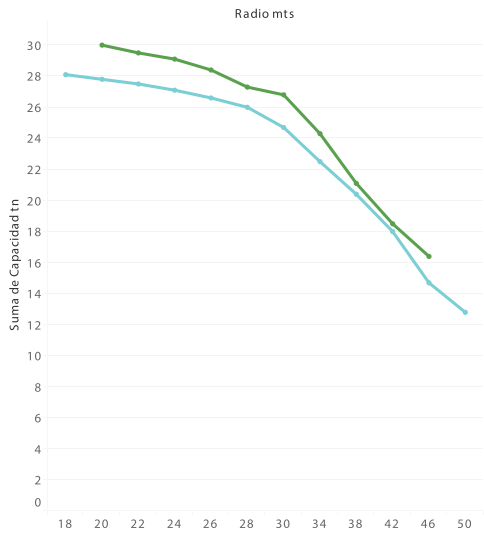
Boom 45.7 m + Luffing 45.7 m (88°) / tn
