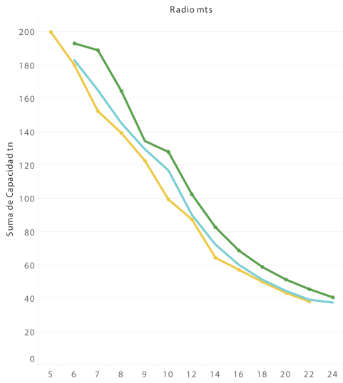
Boom 26 mts / tn
