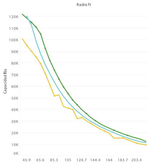
Boom 242.78 ft / lbs
