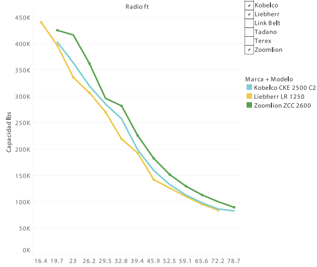
Boom 85.30 ft / lbs
