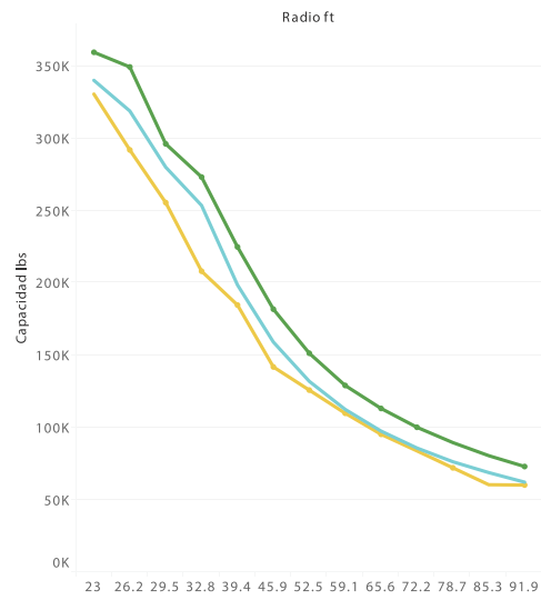
Boom 104.98 ft / lbs
