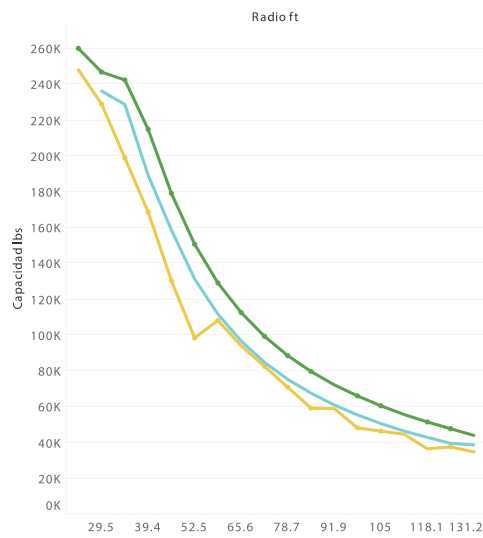
Boom 144.35 ft / lbs
